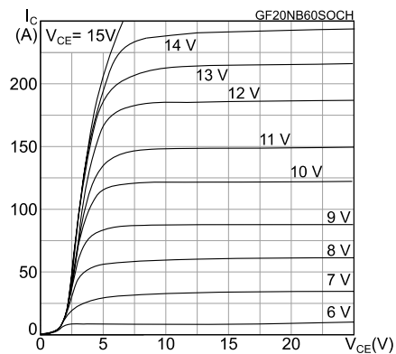
Figure 2: Output Characteristics
