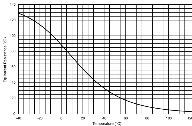
Figure 6. Equivalent resistance ( \text{NTC}/R_{\text{PD\_SD}} )
