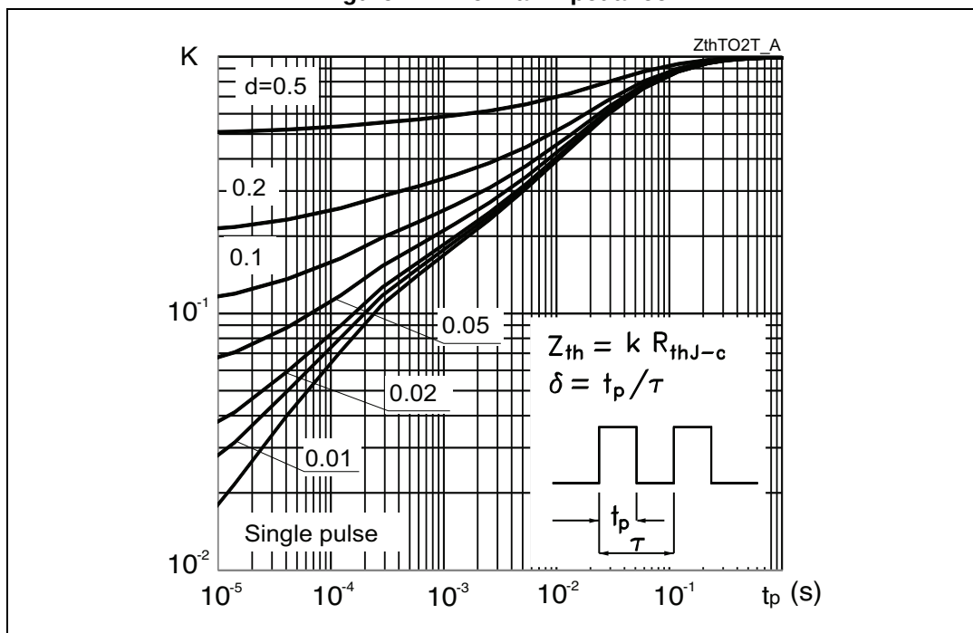
Figure 21. Thermal impedance
