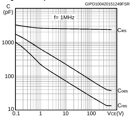
Figure 14: Capacitance variations
