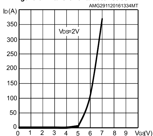
Figure 6: Transfer characteristics
