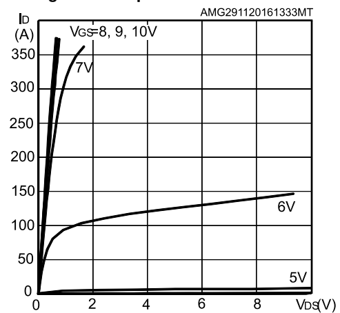
Figure 5: Output characteristics
