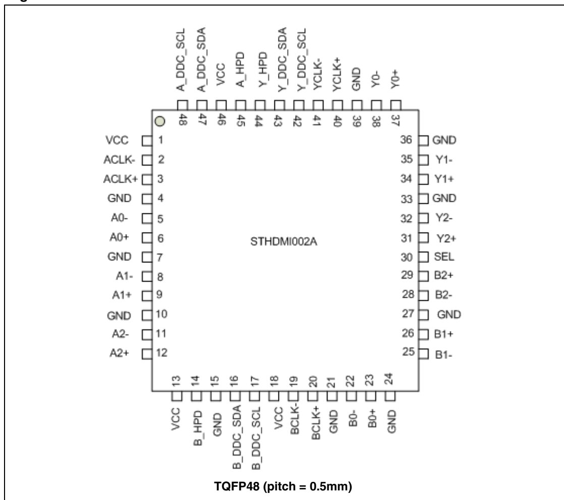
Figure 3. Pin connections
