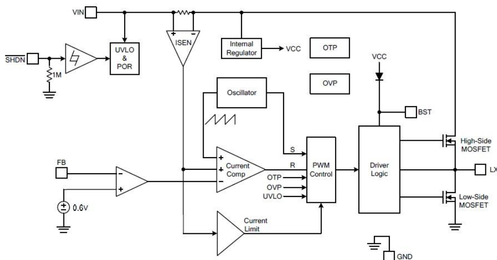
Figure 2. STI3472 Block Diagram
