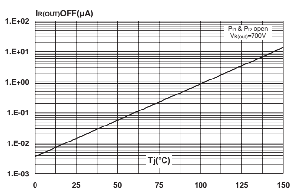
Fig. 5-1: Reverse current versus junction temperature without driver current (typical values).
