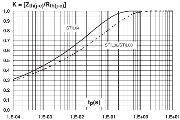
Figure 13: Relative variation of thermal impedance junction to case versus pulse duration
