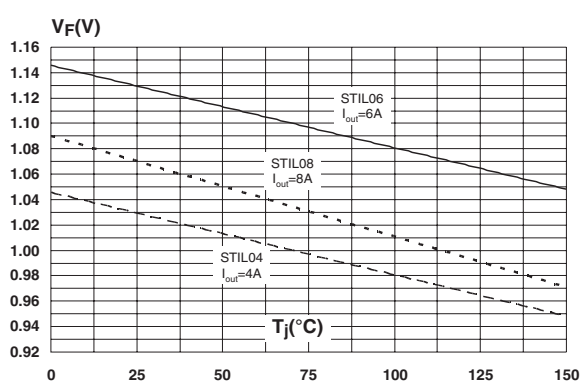
Figure 18: Forward voltage drop for one power switch versus junction temperature (typical values)
