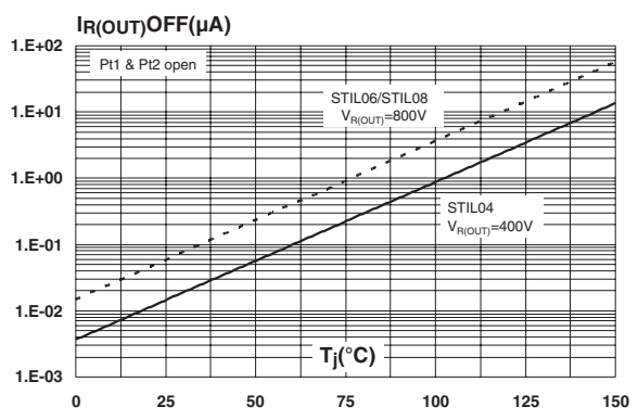
Figure 14: Reverse current versus junction temperature without driver current (typical values)
