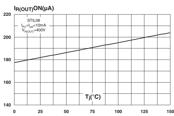
Figure 17: Reverse current versus junction temperature with driver current (typical values) (STIL08)
