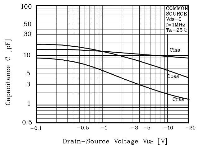
Fig6 C - VDS
