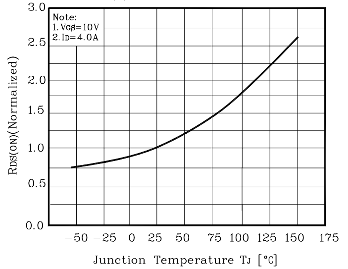
Fig. 8 R_{DS(on)} - T_J
