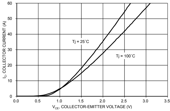
Figure 11. V_{CE} versus I_C for different temperatures ( V_{DD} = 15\text{ V} )
