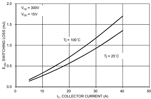
Figure 13. E_{ON} versus I_C for different temperatures
