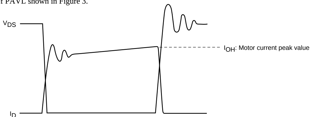
Figure 2 Output Current, I_D , and Voltage, V_{DS} , Waveforms 2 of the STK672-2** Series when Driving a 2-Phase Stepping Motor with Constant Current Chopping
