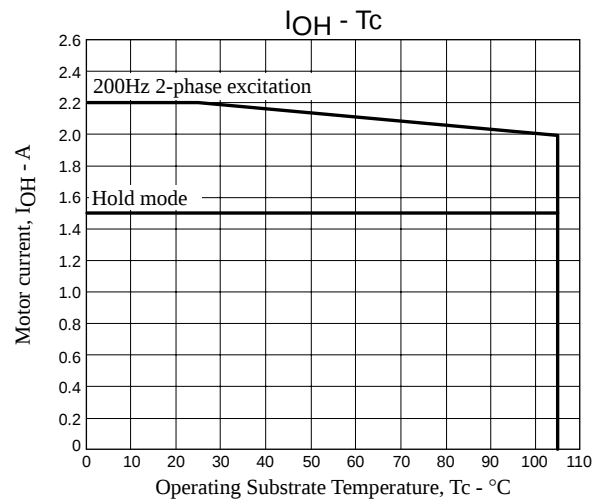
Derating Curve of Motor Current, I_{OH} , vs. STK672-401C-E Operating Substrate Temperature, T_c
