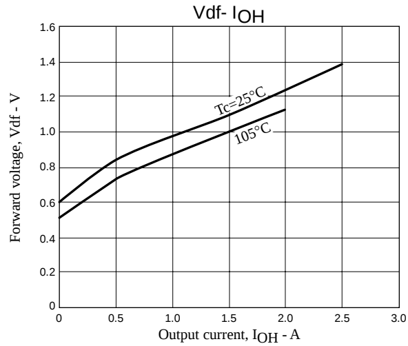
STK672-401C-E Forward voltage, V_{df} - Output current, I_{OH}
