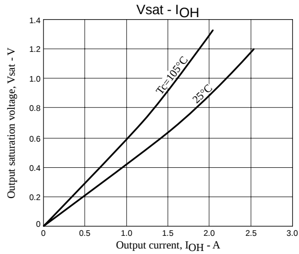
STK672-401C-E Output saturation voltage, V_{sat} - Output current, I_{OH}
