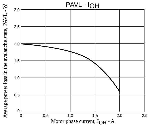
Figure 3 Allowable Loss Range, PAVL - I_{OH} During STK672-401C-E Avalanche Operations
