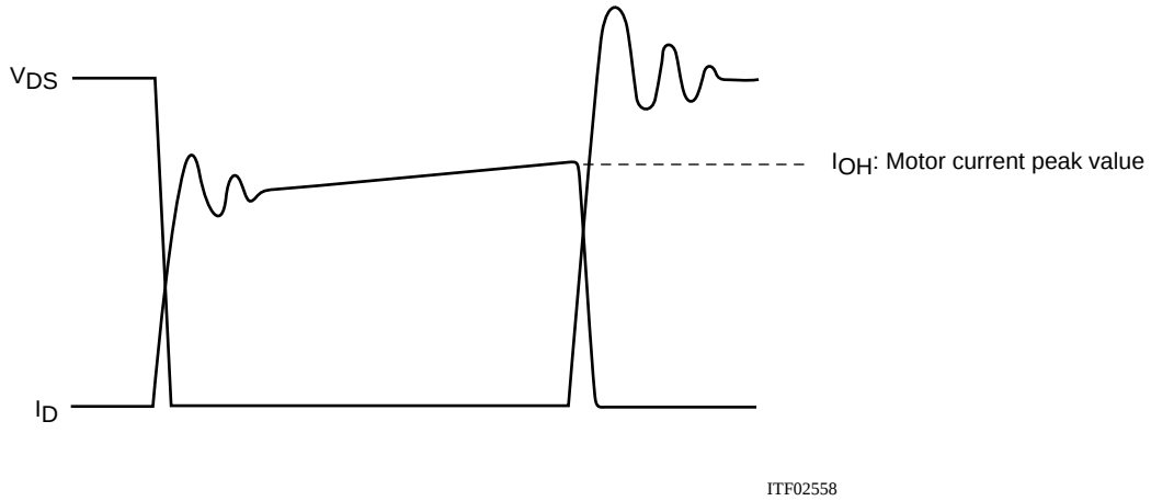
Figure 2 Output Current, I_D , and Voltage, V_{DS} , Waveforms 2 of the STK672-401C-E when Driving a 2-Phase Stepping Motor with Constant Current Chopping
