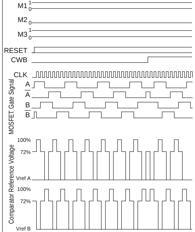
1-2 Phase Excitation Timing Chart (M3=1)
