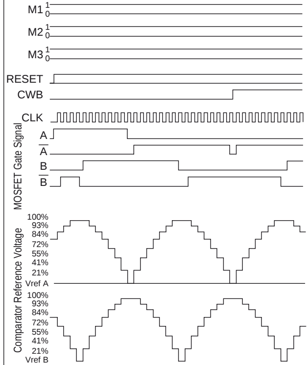
2W1-2 Phase Excitation Timing Chart (M3=1)
