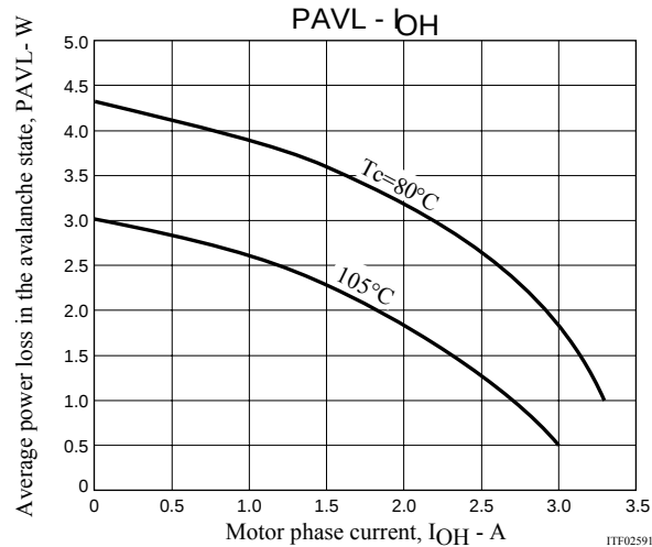
Figure 3 Allowable Loss Range, PAVL-I_{OH} During STK672-640C-E Avalanche Operations
