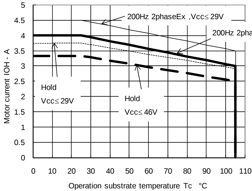
Derating Curve of Motor Current, I_{OH} , vs. STK672-640CN-E Operating Substrate Temperature, T_c
