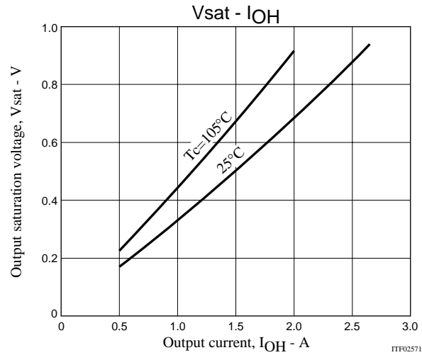
STK672-730A-E Output saturation voltage, V_{sat} - Output current, I_{OH}
