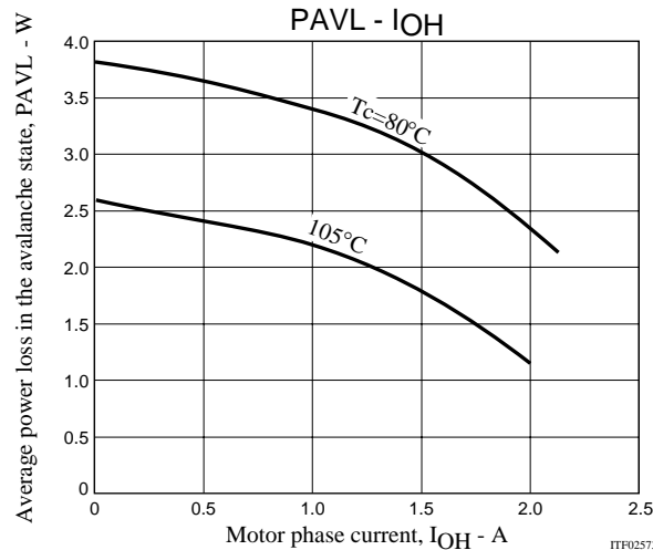
Figure 3 Allowable Loss Range, PAVL-I_{OH} During STK672-730A-E Avalanche Operations
