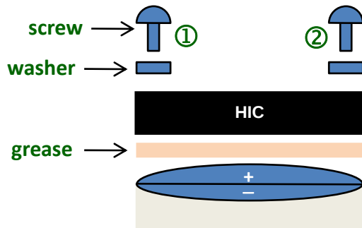
Fig 1 : mount HIC on a Heat Sink
