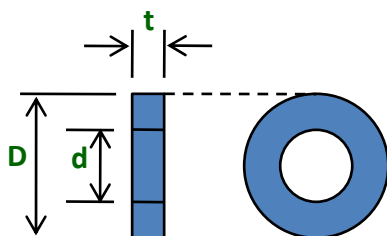
Fig 2 : size of washer
