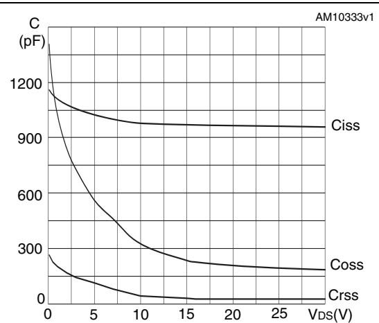
Figure 9. Capacitance variations
