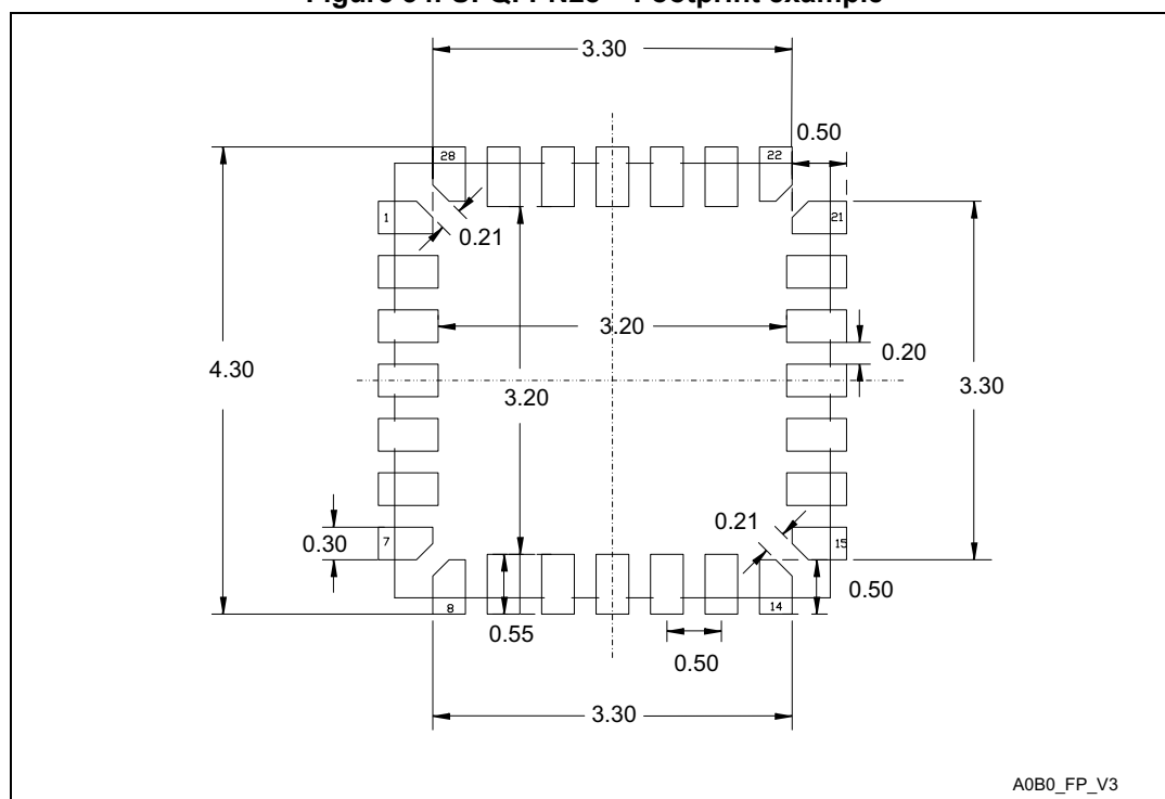
Figure 34. UFQFPN28 – Footprint example
