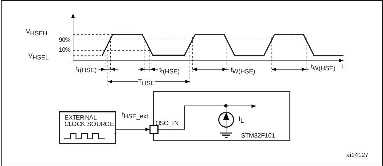
Figure 10. High-speed external clock source AC timing diagram
