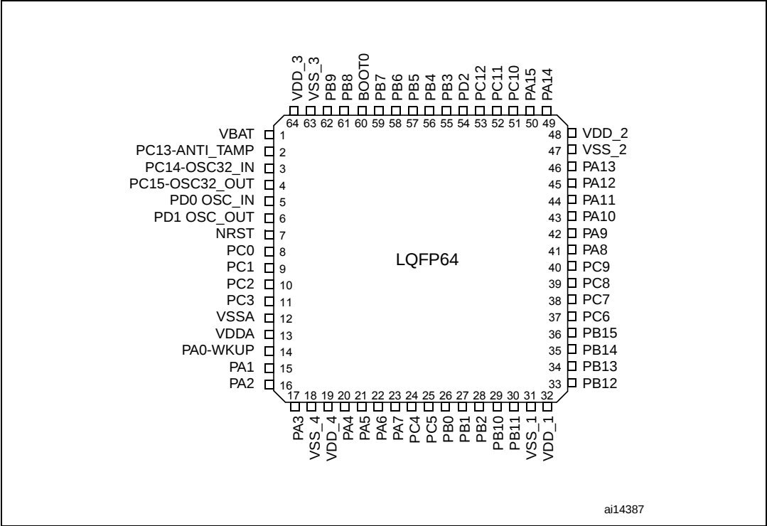
Figure 3. STM32F101xx access line LQFP64 pinout
