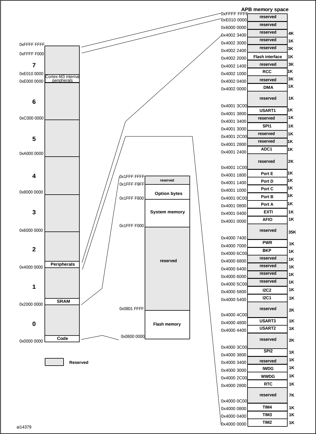
Figure 5. Memory map
