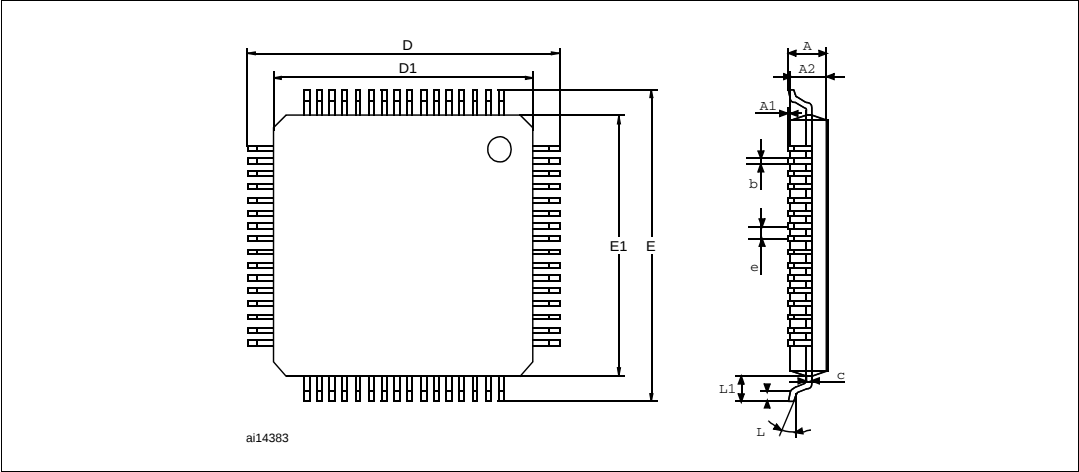
Figure 26. LQFP64 – 64-pin low-profile quad flat package outline
