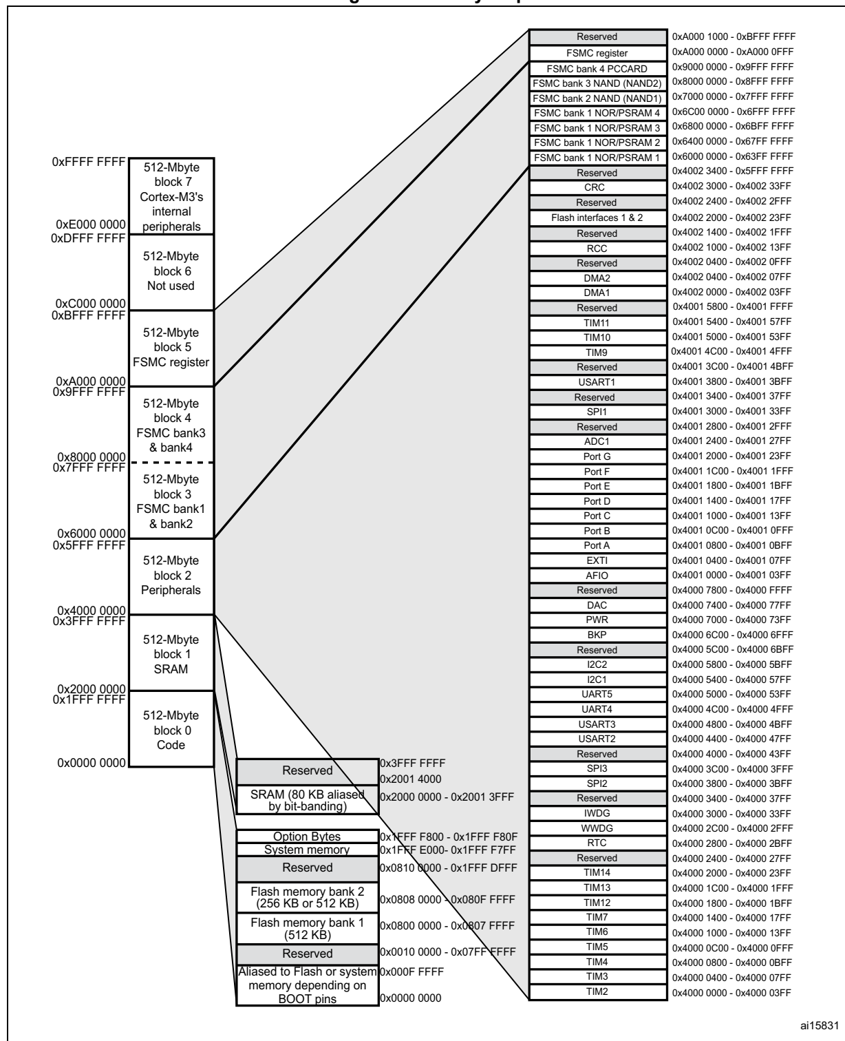
Figure 6. Memory map
