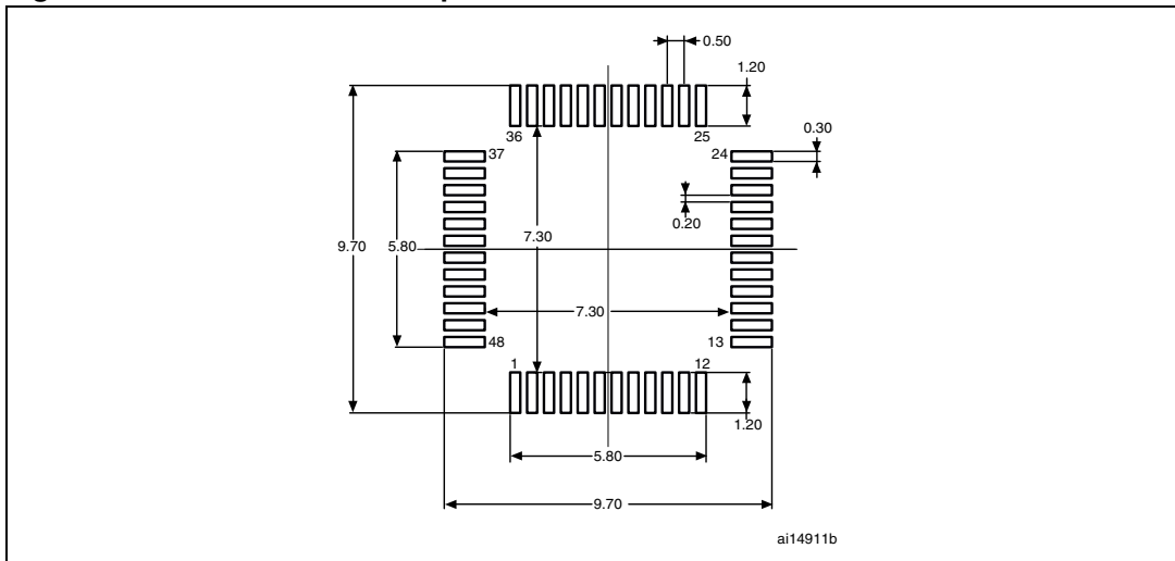
Figure 37. Recommended footprint
