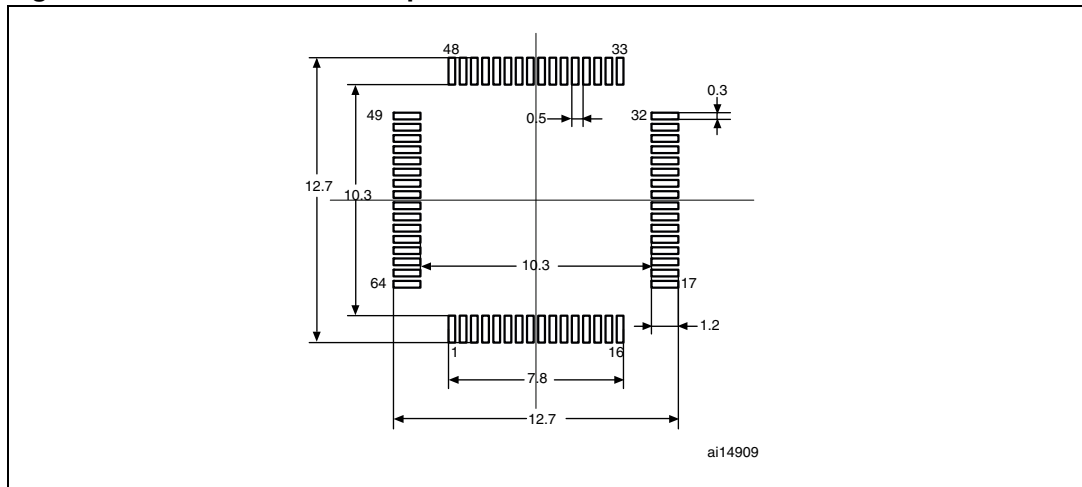
Figure 35. Recommended footprint
