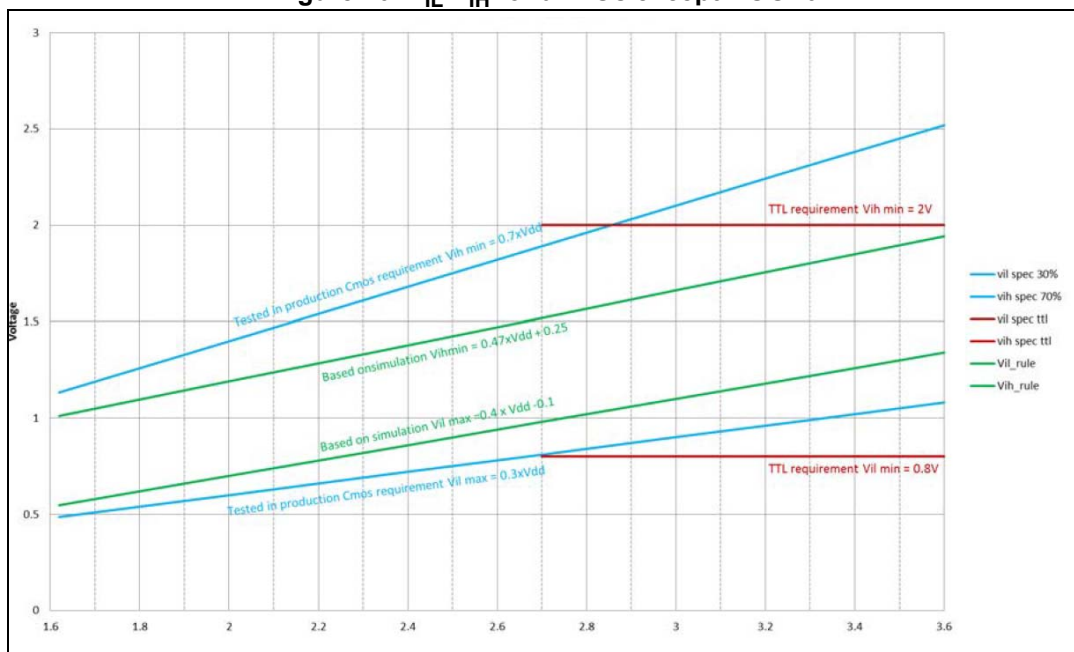
Figure 20. V_{IL}/V_{IH} for all I/Os except BOOT0
