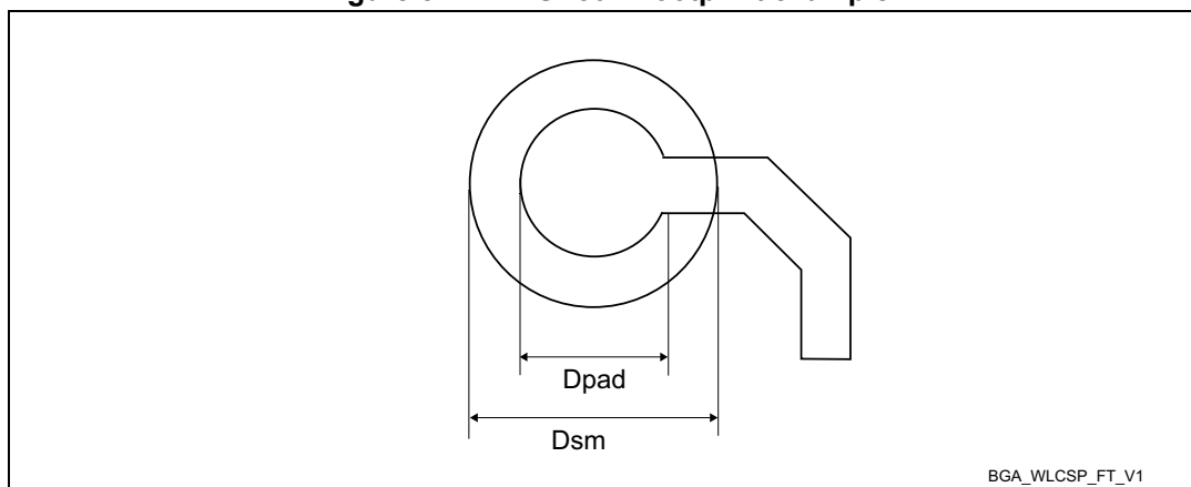
Figure 84. WLCSP80 - Footprint example
