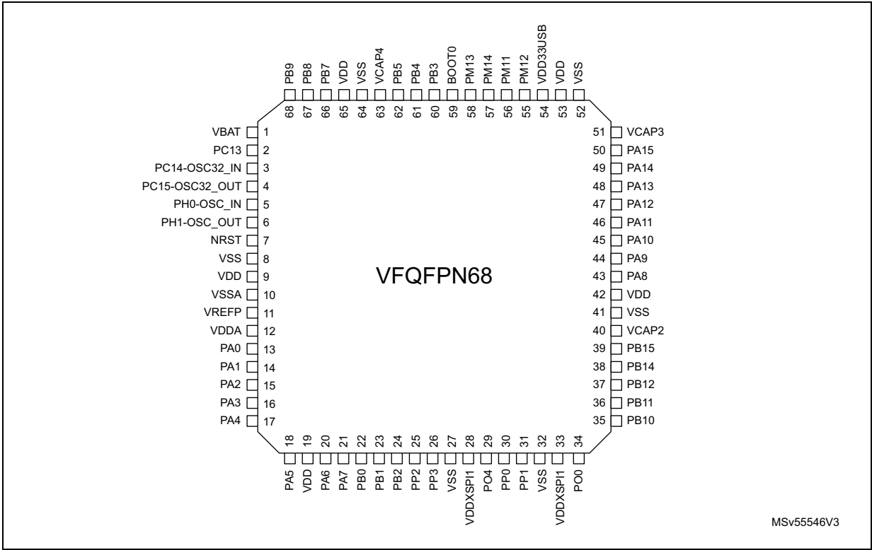
Figure 18. VFQFPN68 GP pinout(a)
