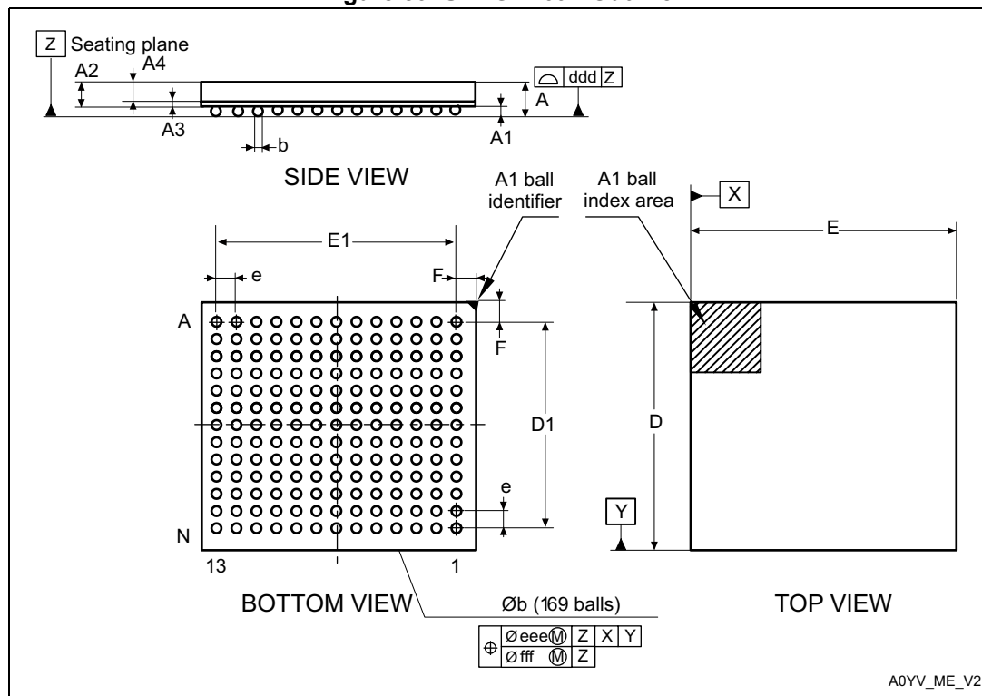
Figure 89. UFBGA169 - Outline
