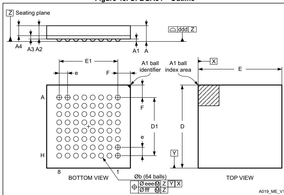
Figure 48. UFBGA64 – Outline
