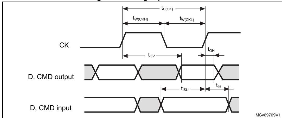
Figure 45. SD default mode
