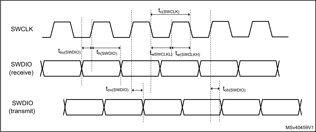
Figure 52. SWD timing
