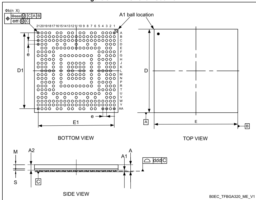
Figure 57. TFBGA320 - Outline
