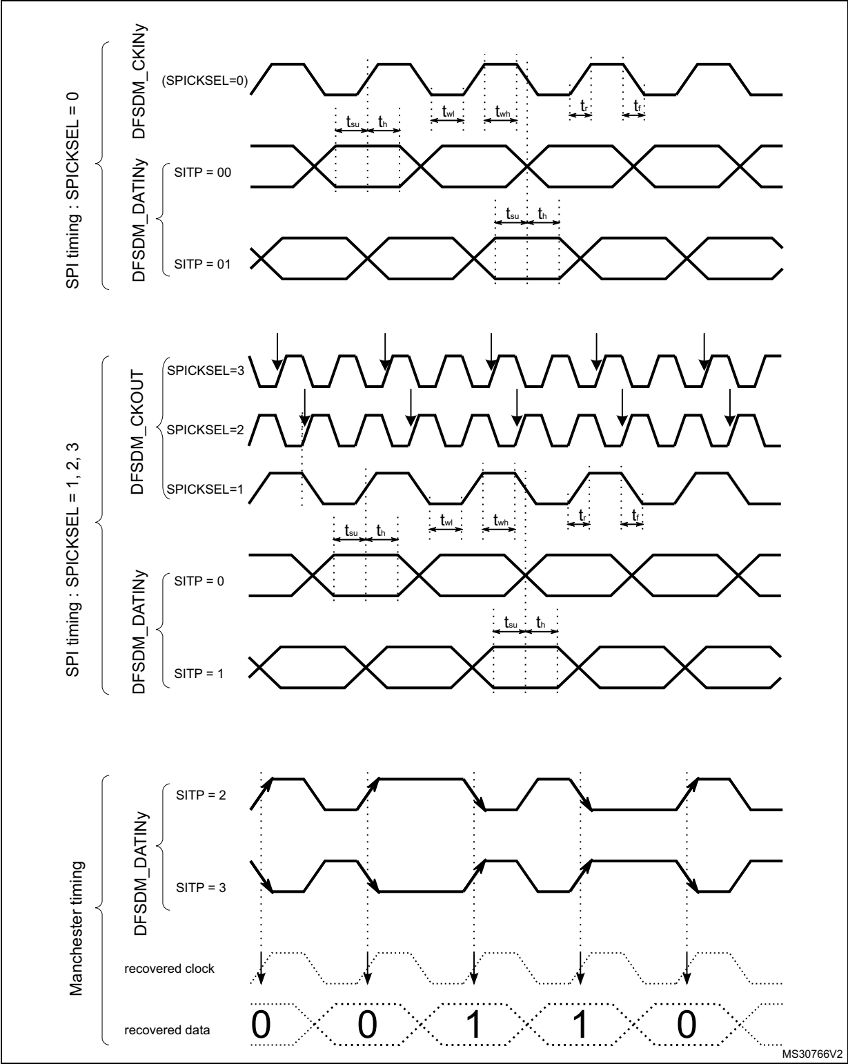
Figure 38. Channel transceiver timing diagrams
