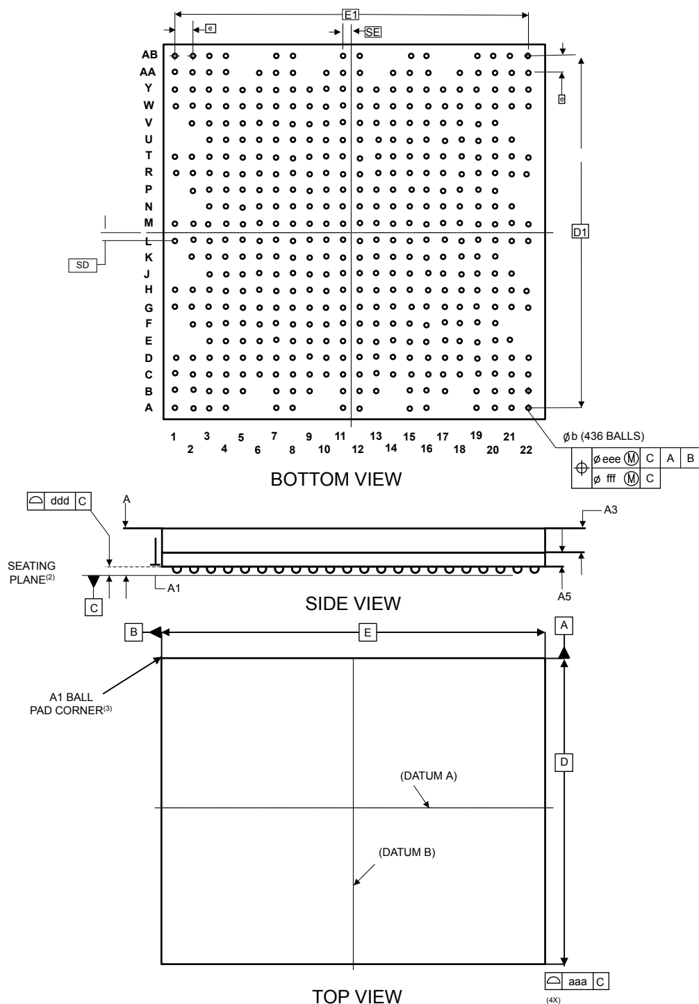
Figure 67. TFBGA436 - Outline
