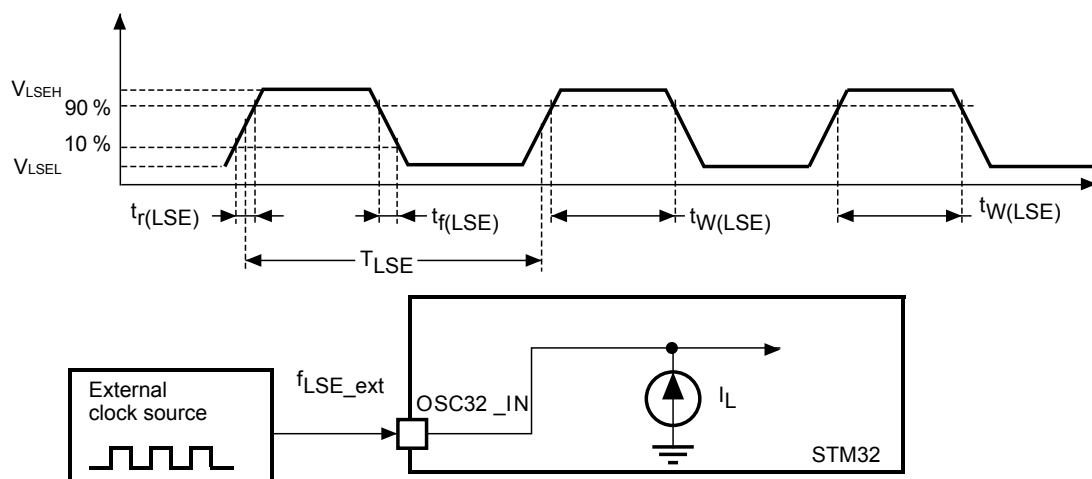
Figure 15. Low-speed external clock source AC timing diagram (digital bypass)
