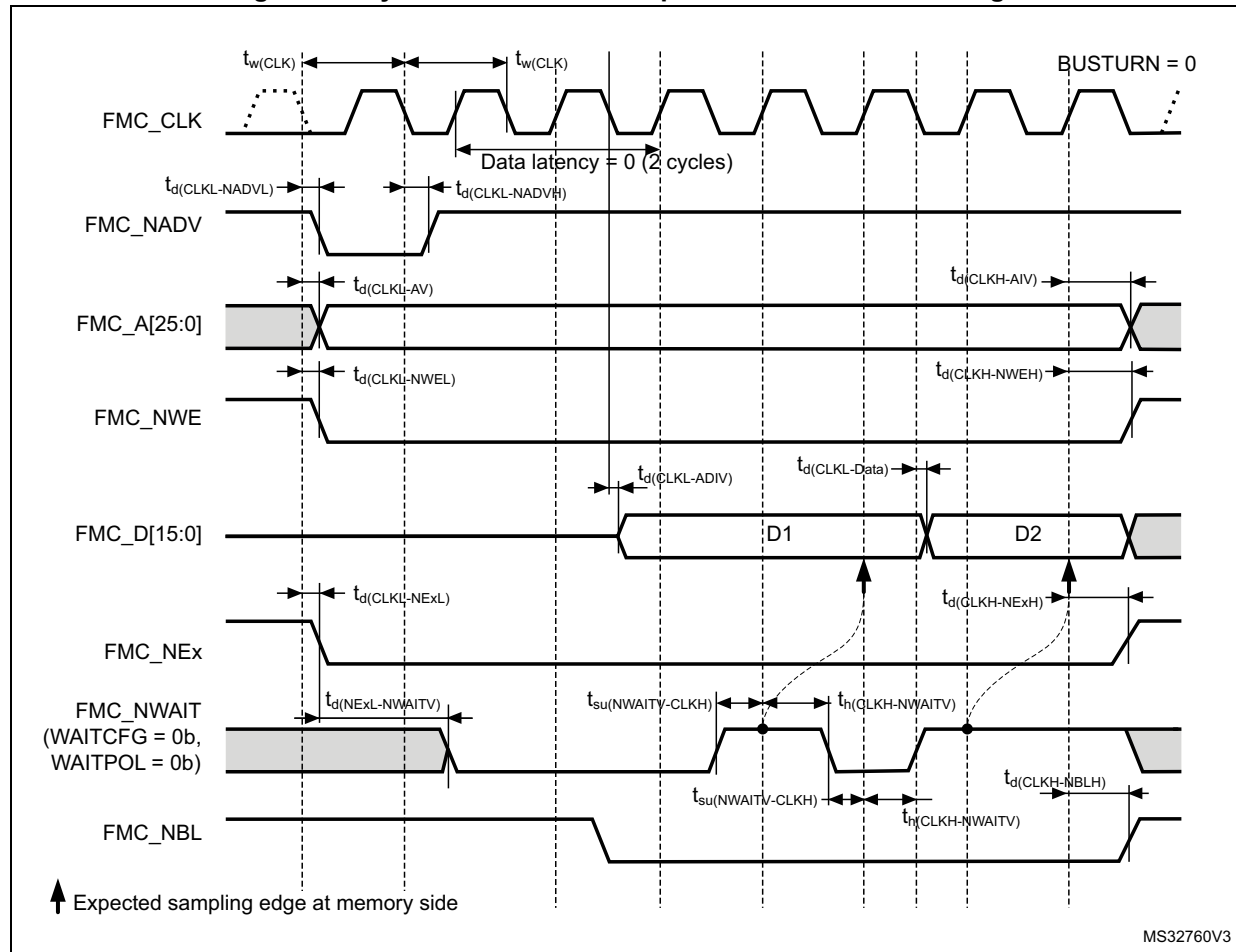
Figure 30. Synchronous non multiplexed PSRAM write timings
