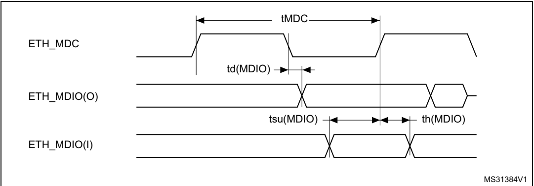
Figure 61. Ethernet MDIO/SMA timing diagram
