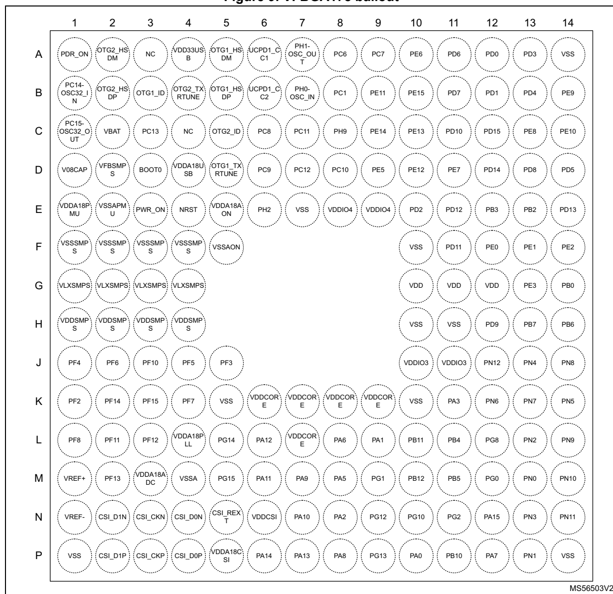
Figure 9. VFBGA178 ballout
