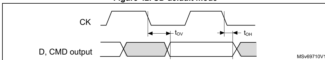
Figure 42. SD default mode
