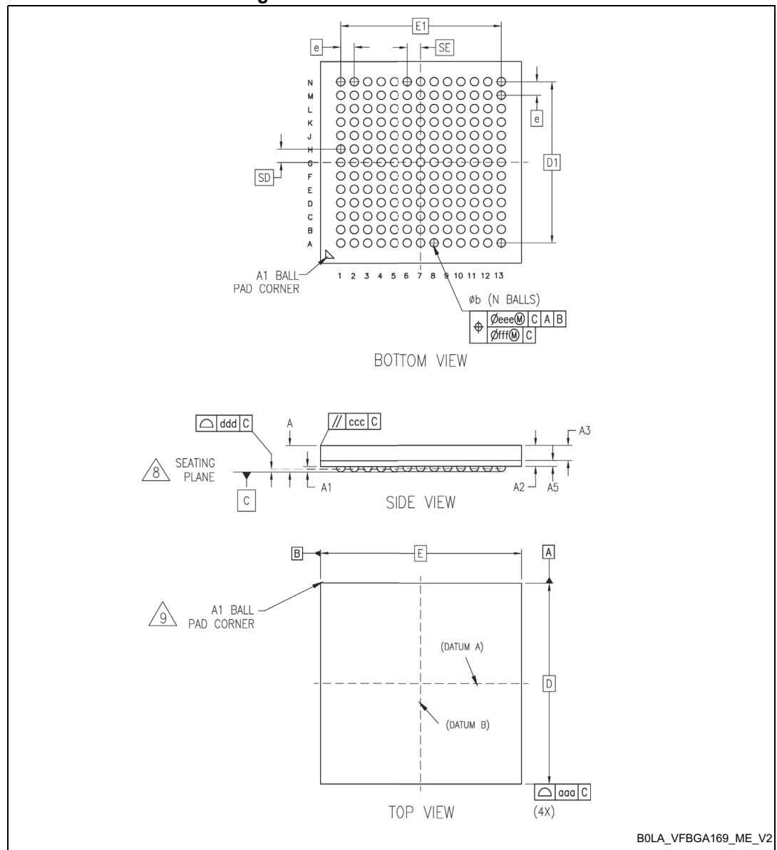
Figure 67. VFBGA169 - Outline (13)
