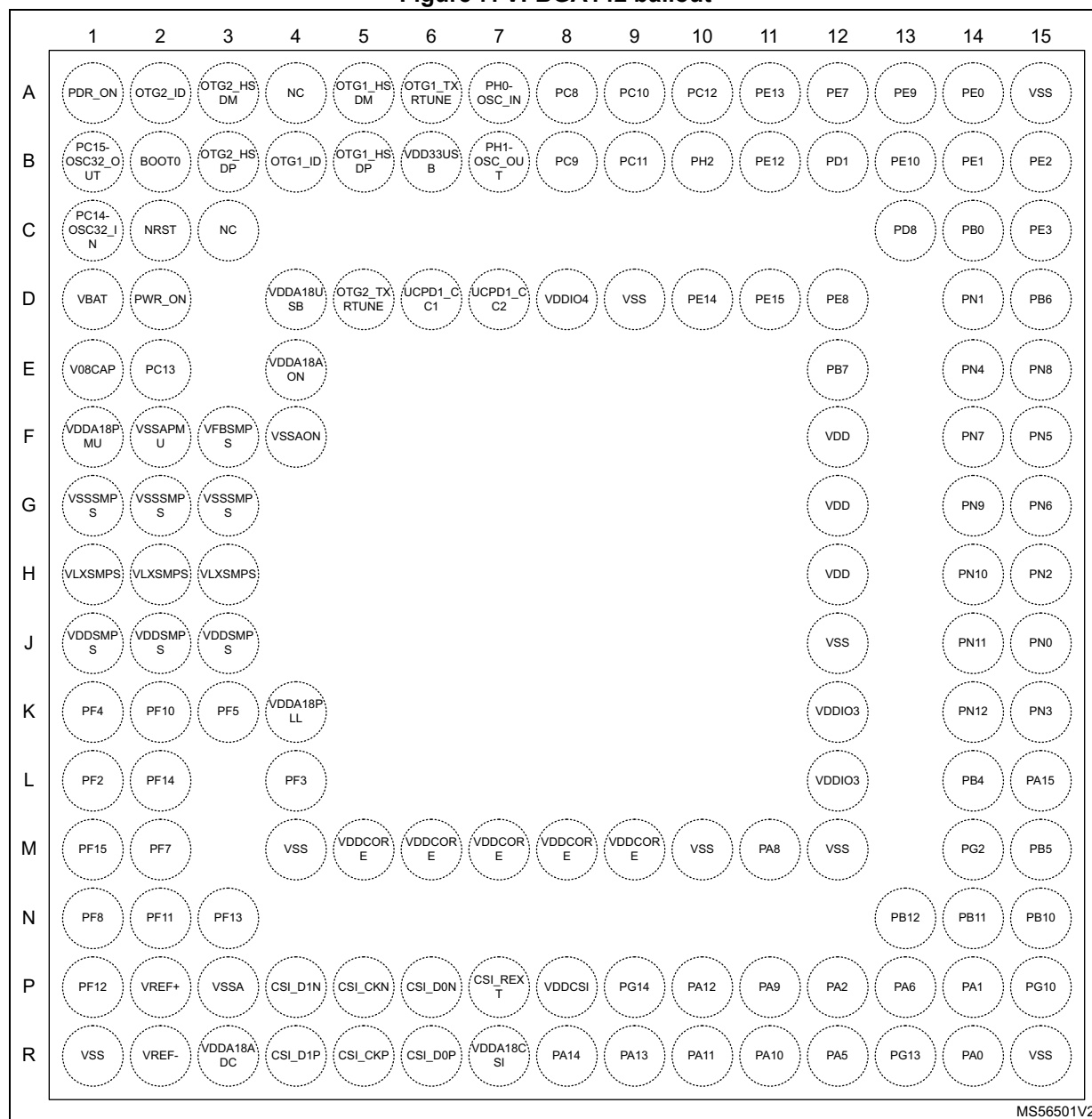
Figure 7. VFBGA142 ballout
