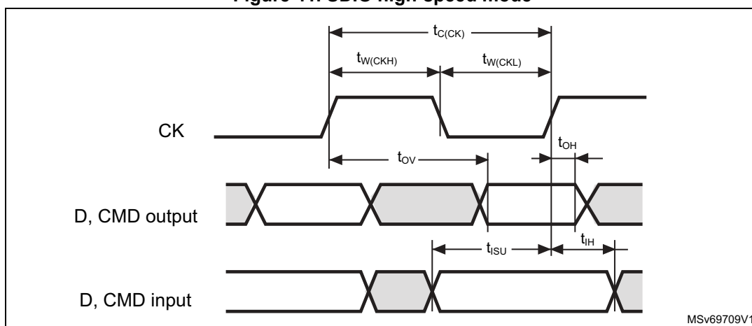
Figure 41. SDIO high-speed mode
