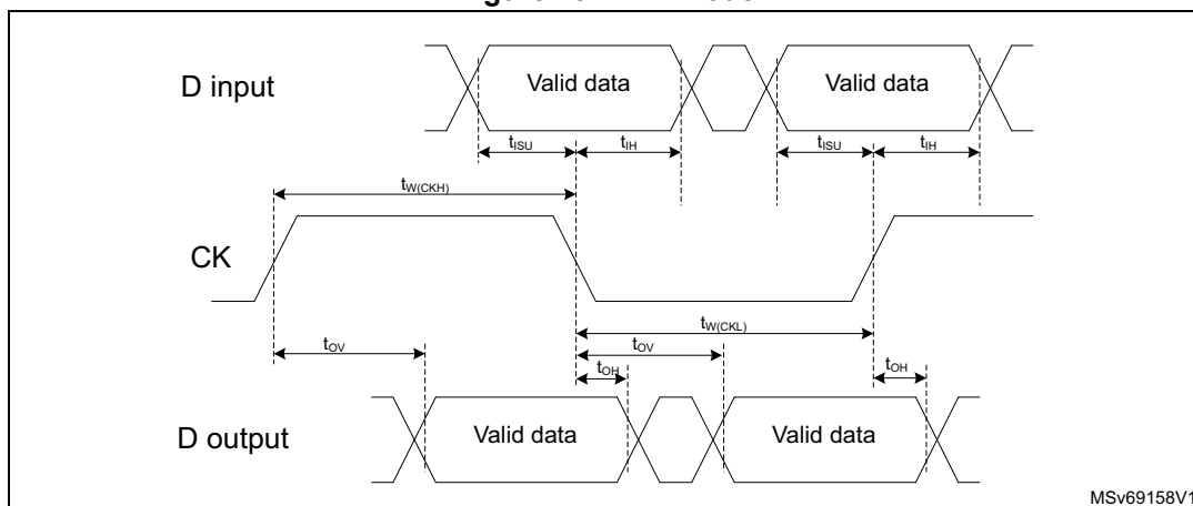
Figure 43. DDR mode
