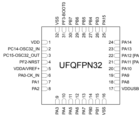
Figure 3. UFQFPN32 pinout
