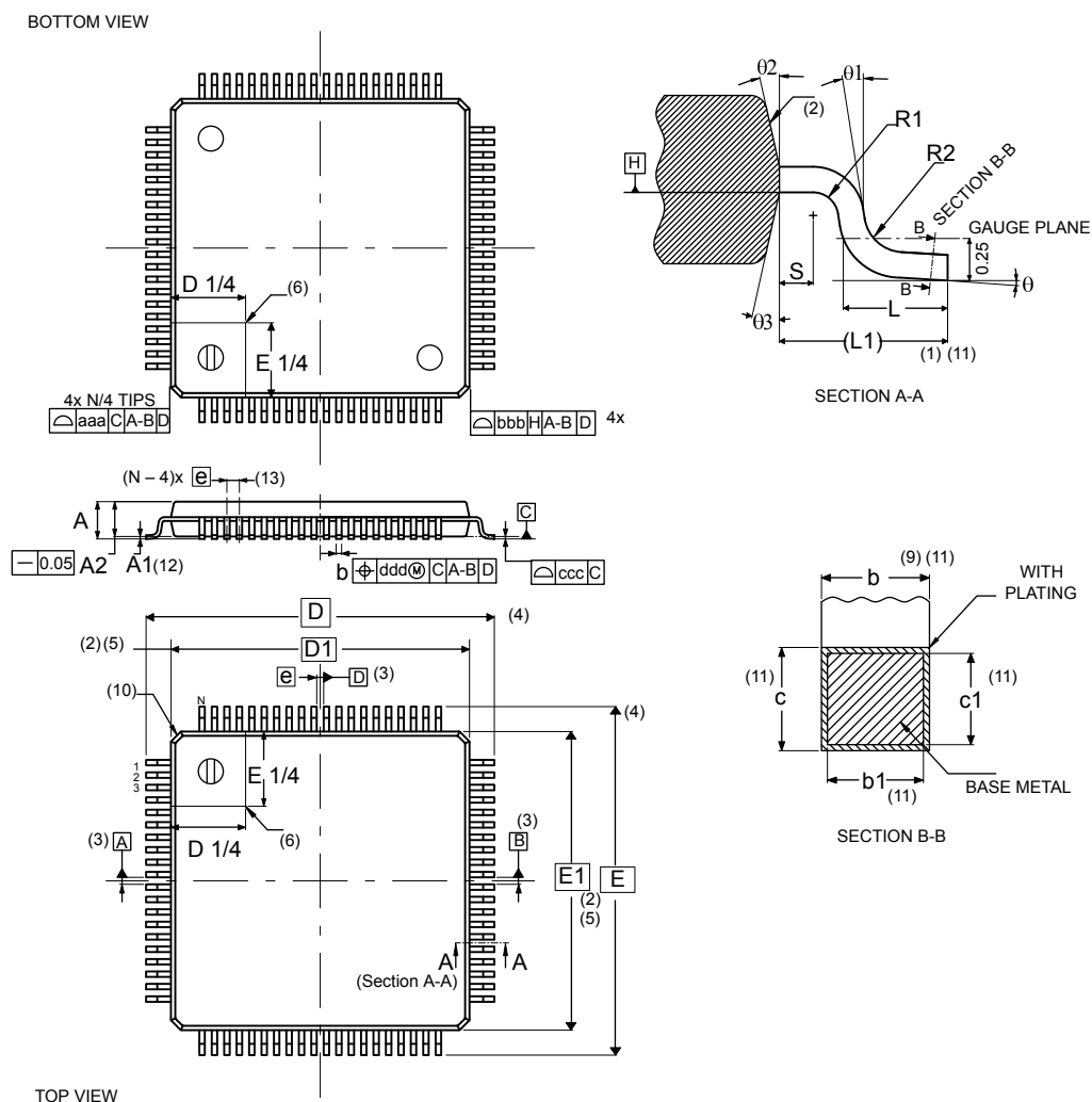
Figure 47. LQFP80 - Outline (15.)
