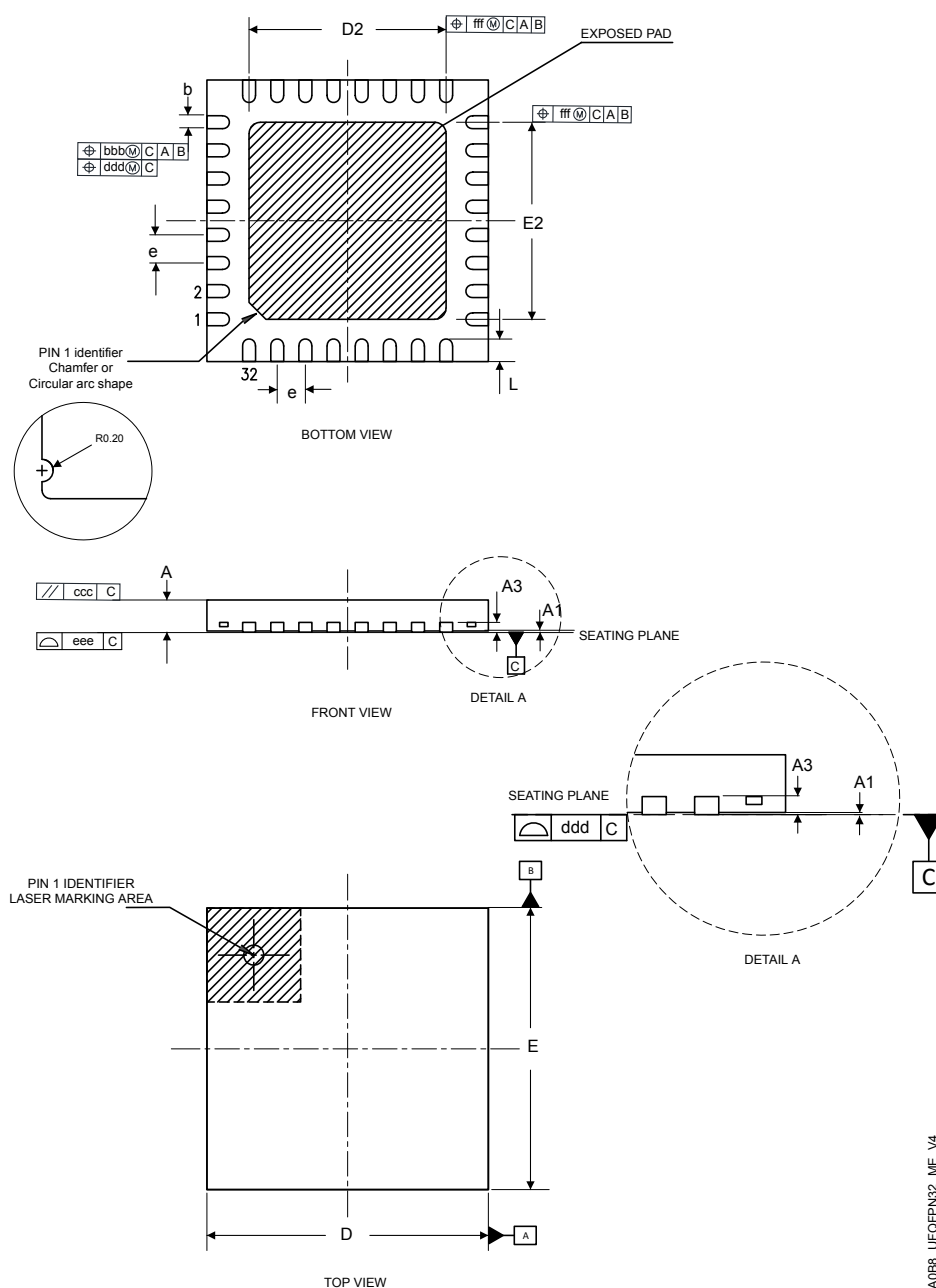
Figure 34. UFQFPN32 - Outline
