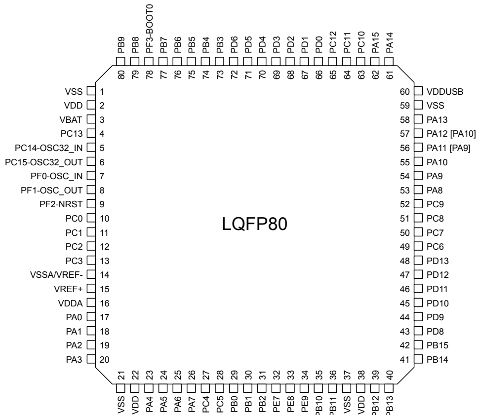
Figure 9. LQFP80 pinout
