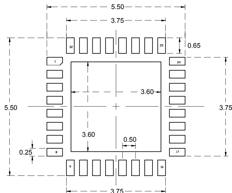
Figure 35. UFQFPN32 - Footprint example
