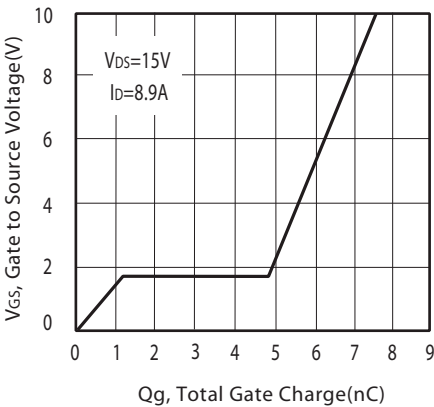
Figure 10. Gate Charge
