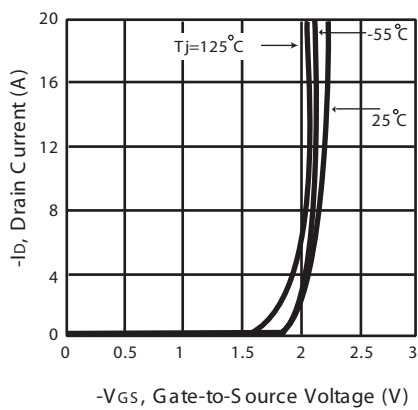
Figure 2. Transfer Characteristics
