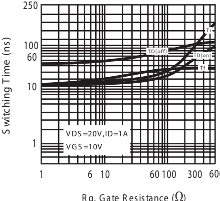
Figure 11. switching characteristics
