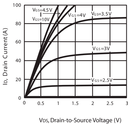
Figure 1. Output Characteristics
