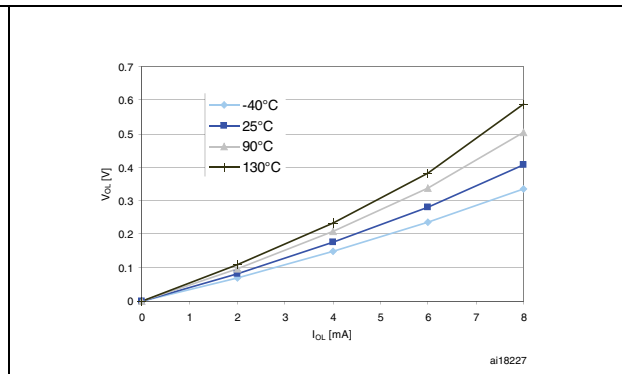
Figure 18. Typ. V_{OL} @ V_{DD} = 1.8 V (standard ports)
