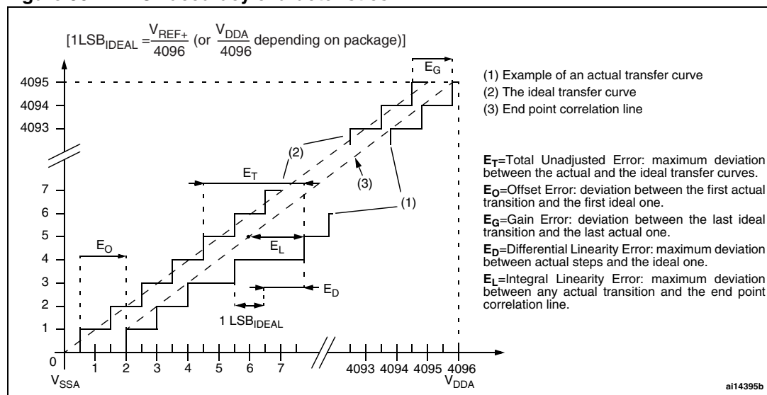
Figure 30. ADC1 accuracy characteristics
