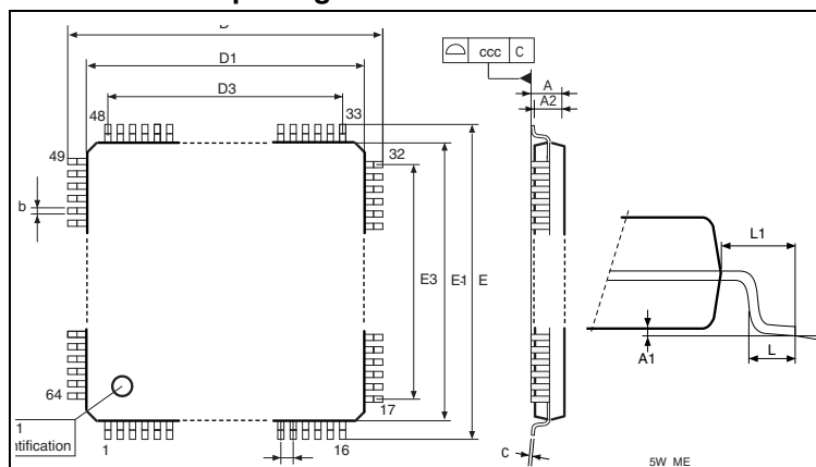
Figure 35. LQFP64 – 10 x 10 mm, 64 pin low-profile quad flat package outline (1)
