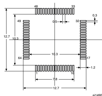
Figure 36. Recommended footprint (1)(2)
