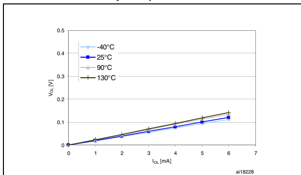
Figure 19. Typ. V_{OL} @ V_{DD} = 3.0 V (true open drain ports)
