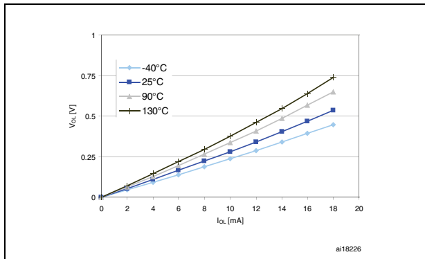
Figure 17. Typ. V_{OL} @ V_{DD} = 3.0 V (standard ports)
