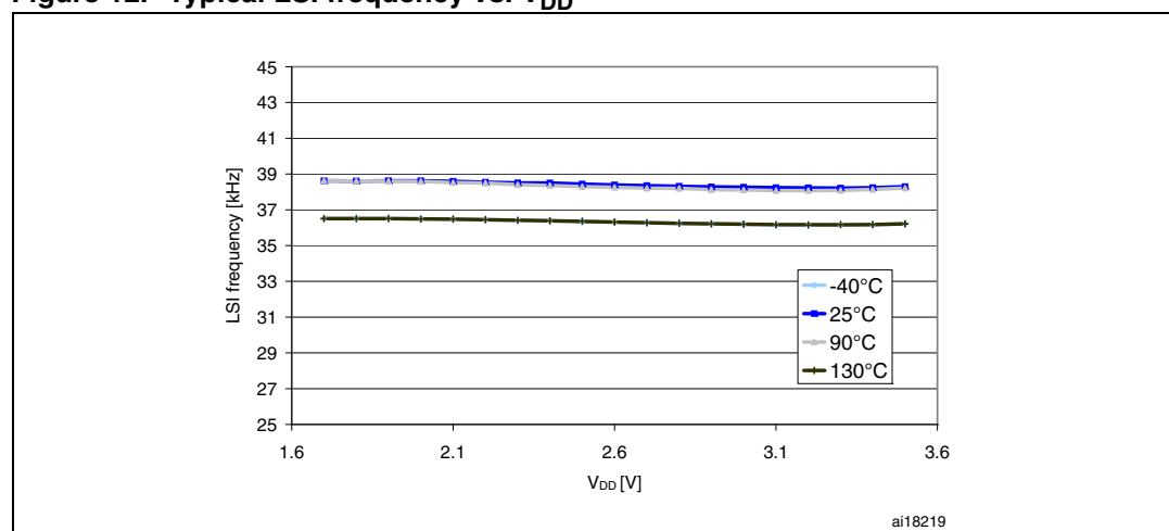
Figure 12. Typical LSI frequency vs. V_{\text{DD}}
