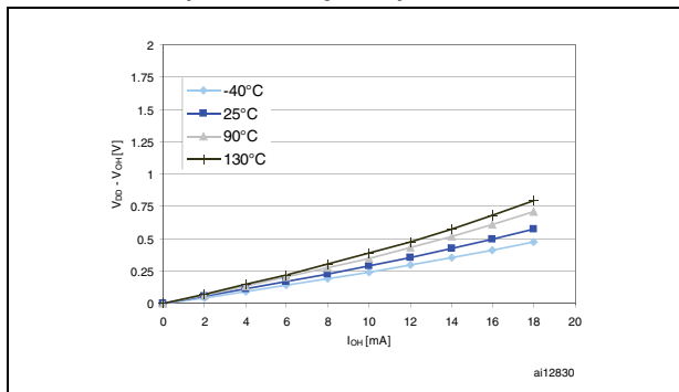
Figure 21. Typ. V_{DD} - V_{OH} @ V_{DD} = 3.0 V (standard ports)
