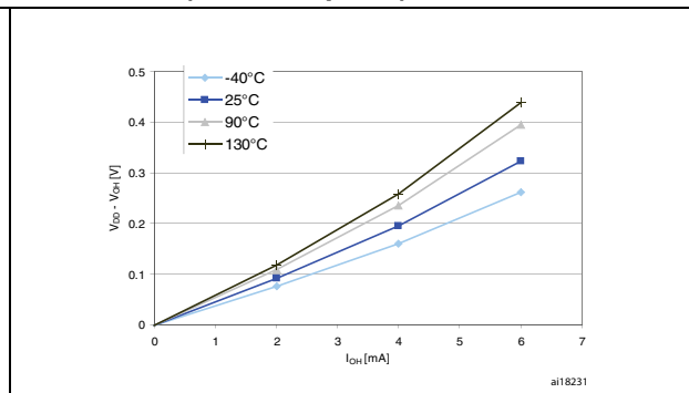
Figure 22. Typ. V_{DD} - V_{OH} @ V_{DD} = 1.8 V (standard ports)
