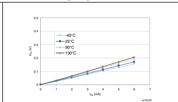
Figure 20. Typ. V_{OL} @ V_{DD} = 1.8 V (true open drain ports)
