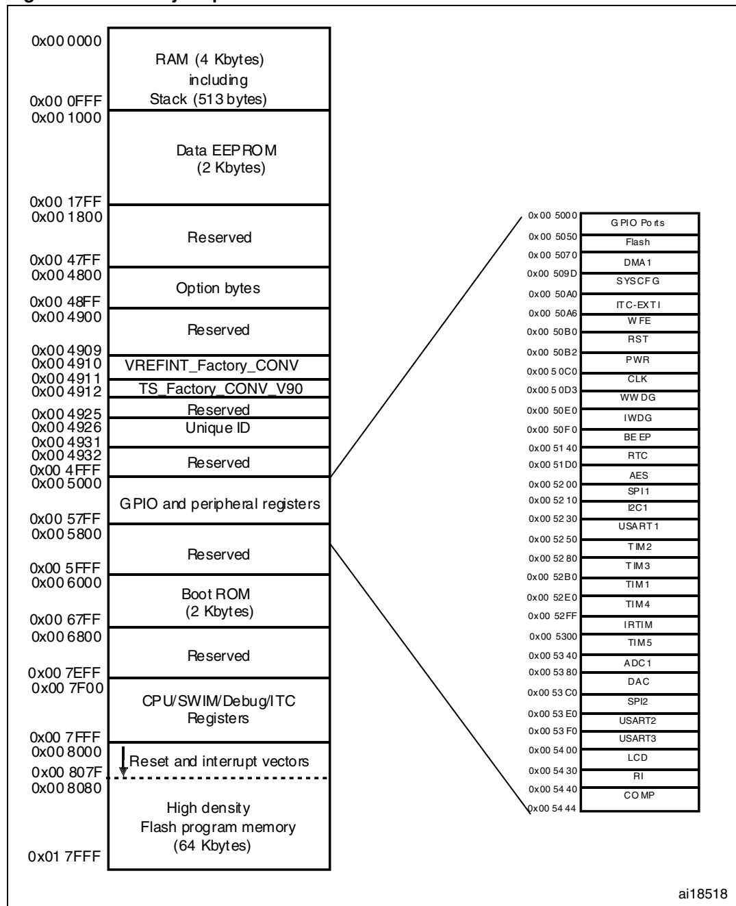
Figure 5. Memory map
