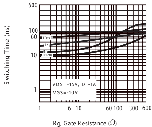
Figure 11. switching characteristics
