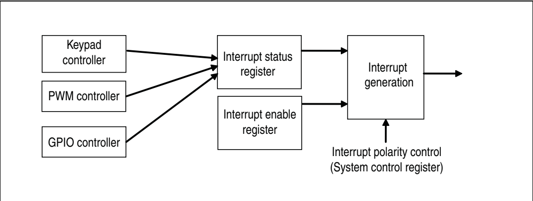
Figure 6. Interrupt system
