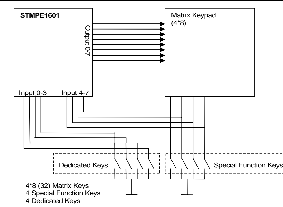
Figure 10. Maximum configuration
