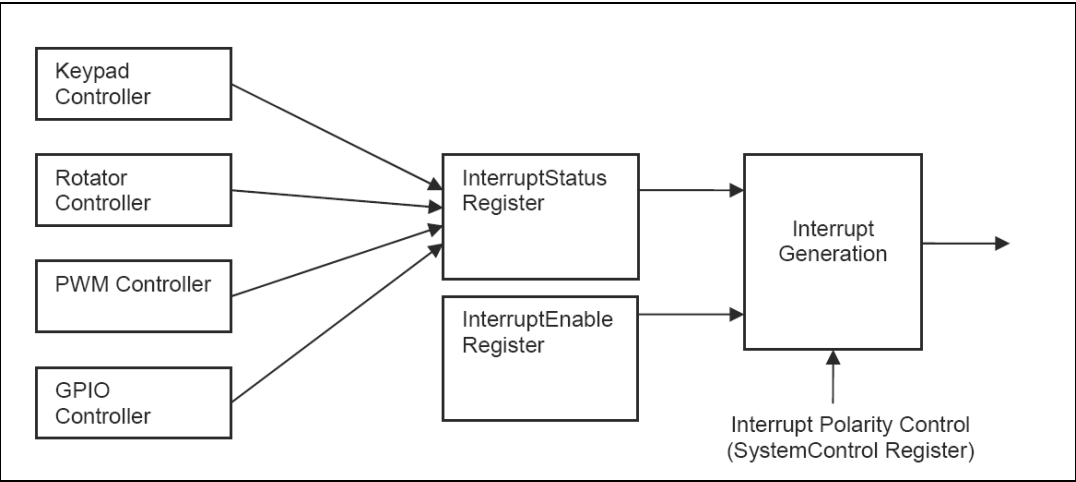
Figure 7. Interrupt system
