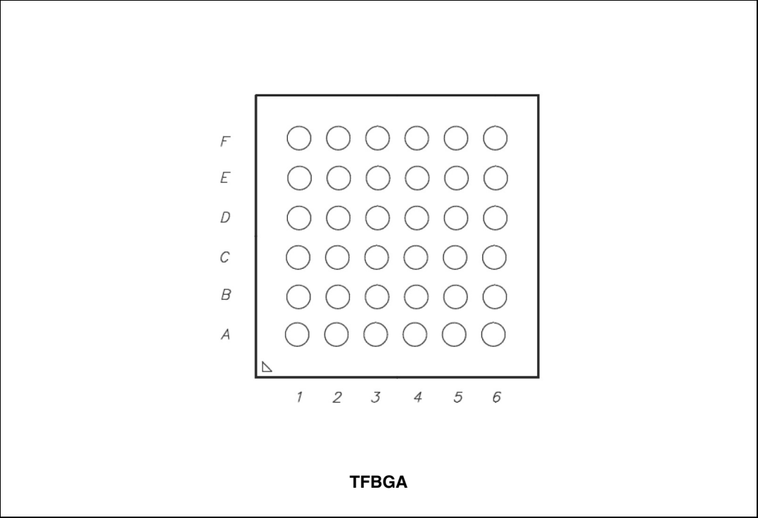
Figure 2. Pin connection
