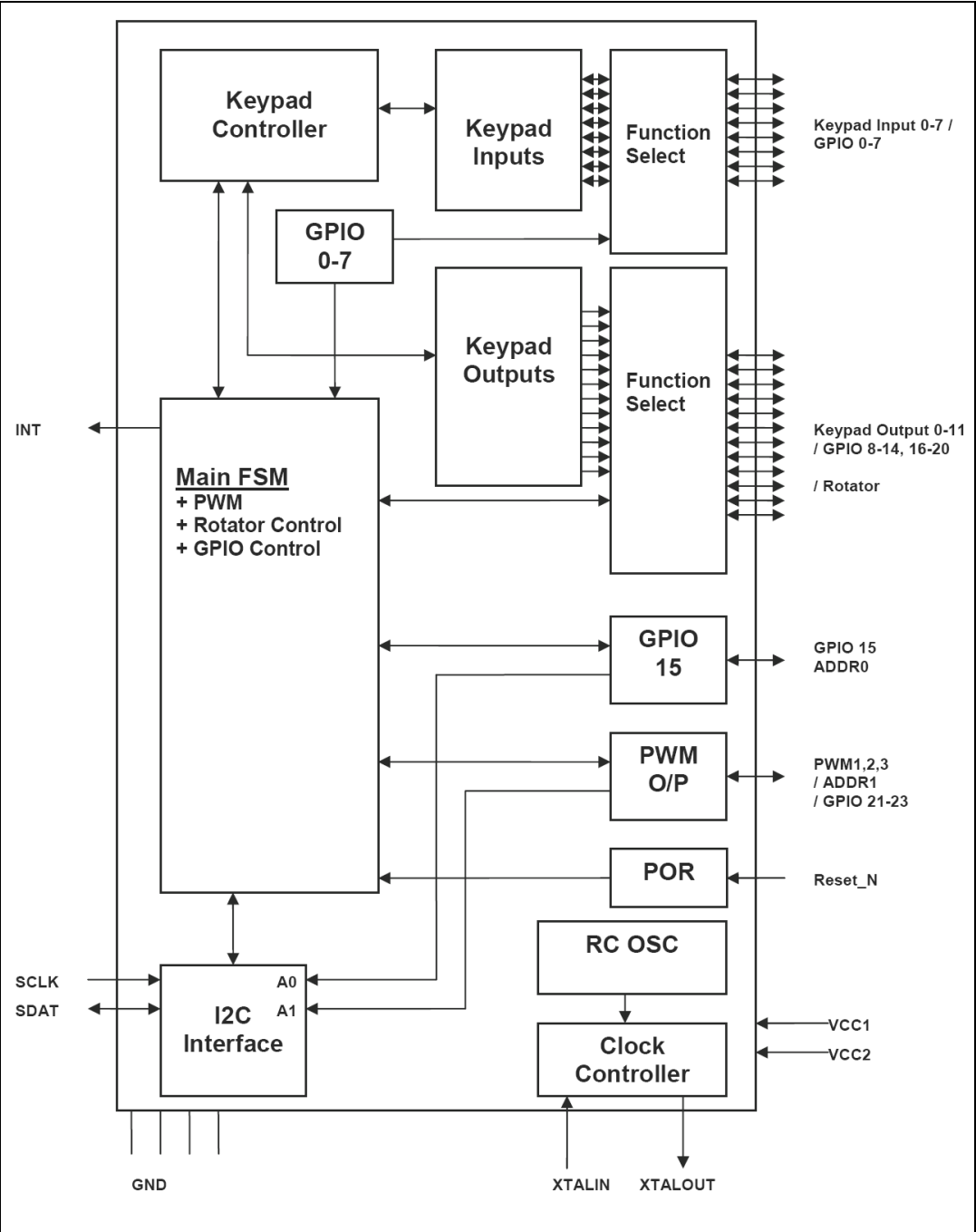
Figure 1. Block diagram
