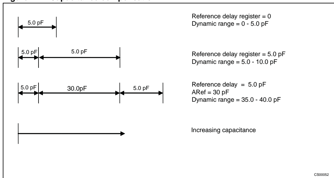
Figure 4. Capacitance compensation
