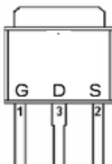
TO-251
