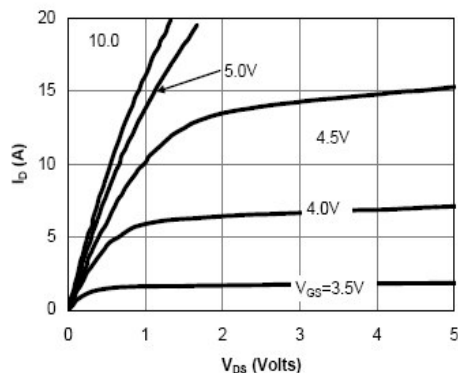
Fig 1: On-Region Characteristics
