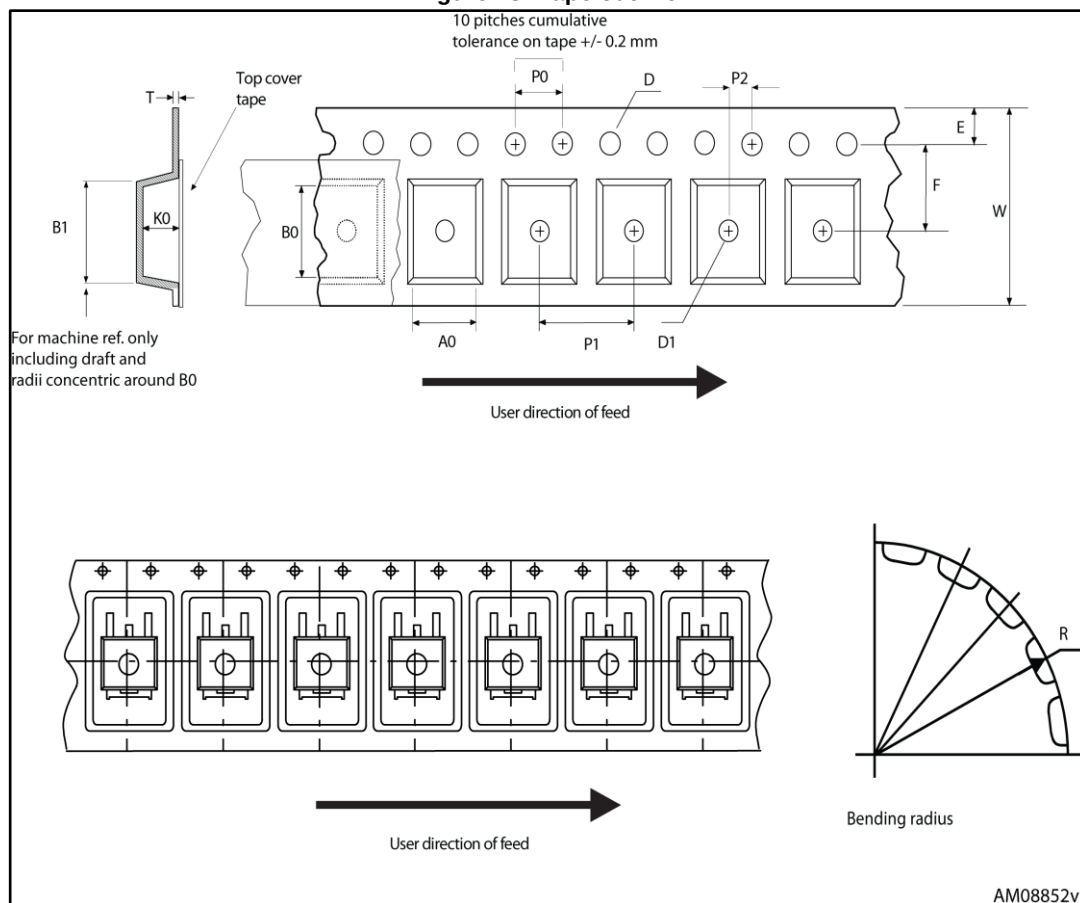
Figure 28: Tape outline
