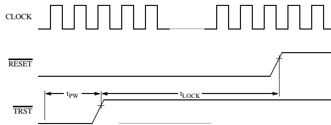
Figure 15. Reset Timing
