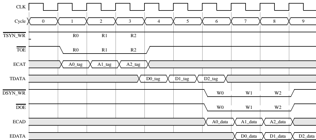
Figure 6. Coherent Write Hit to M State Line
