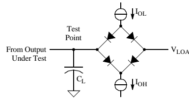
Figure 10. Load Circuit
