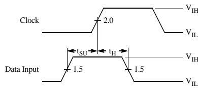
Figure 12. Voltage Waveforms - Setup and Hold Times
