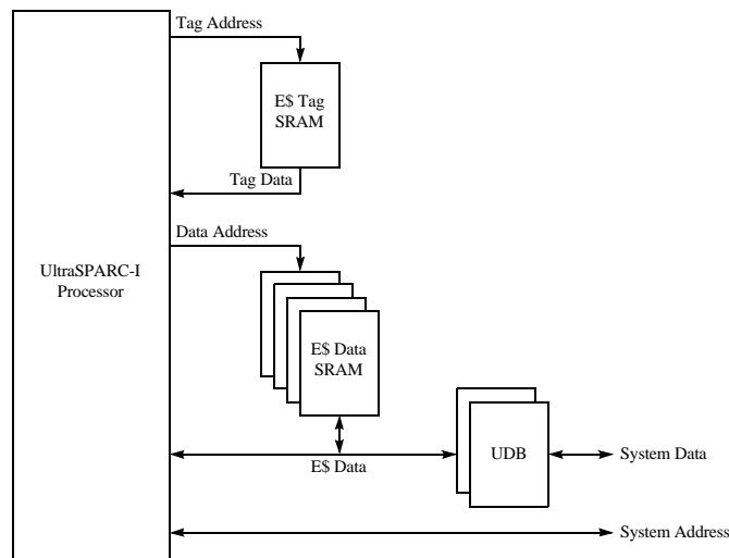
Figure 2. UltraSPARC-I Subsystem System Interface
