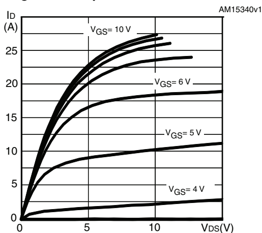
Figure 6. Output characteristics
