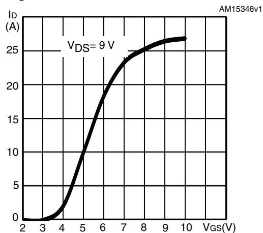
Figure 7. Transfer characteristics
