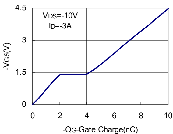
Gate Charge
