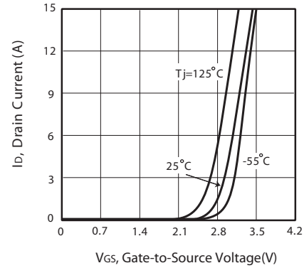
Figure 2. Transfer Characteristics
